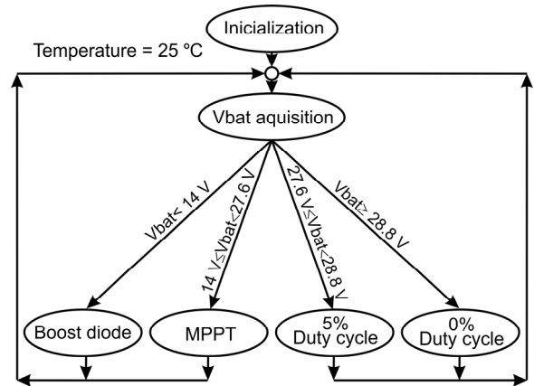
Fig. 10. Routines for charge the batteries.
