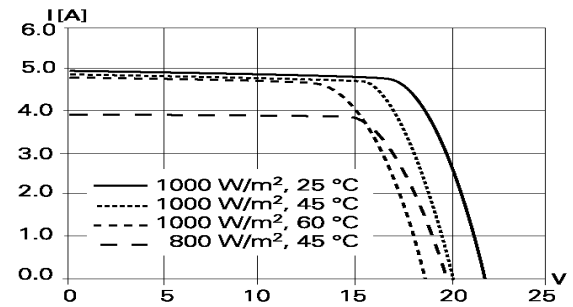
Fig. 7. The I \times V curves of the photovoltaic module obtained from the manufacturer's manual.
