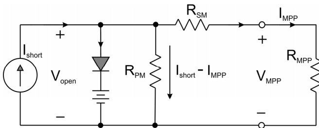
Fig. 4. Equivalent circuit of the module in the maximum power point.
