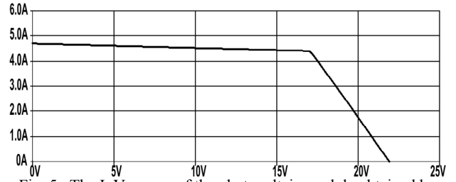
Fig. 5. The I \times V curves of the photovoltaic module obtained by simulation.
