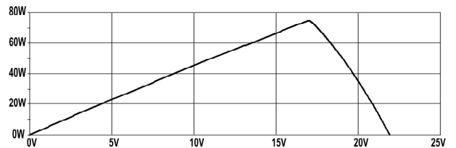
Fig. 6. Simulated P \times V Curve of the photovoltaic module.
