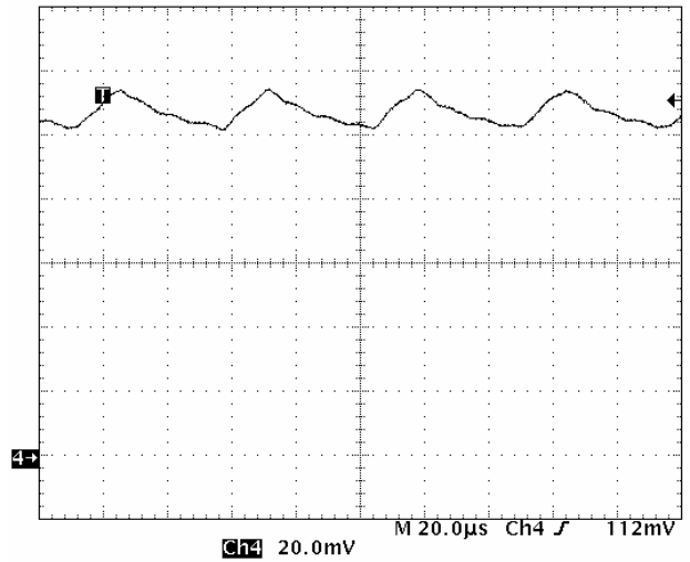
Fig. 17. Battery charge current (200mA/div).
