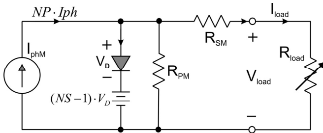
Fig. 3. The electric model for a photovoltaic module with load.
