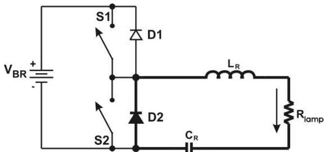
Fig.15.c. Third stage.
