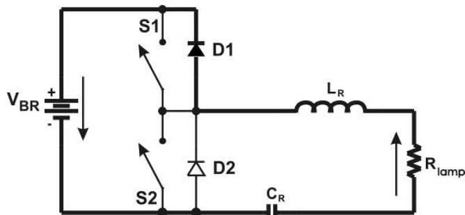
Fig.15.a. First stage.
