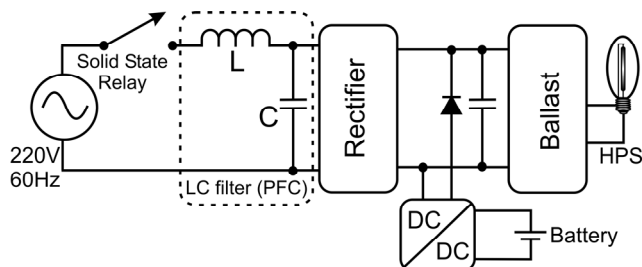
Fig. 13. HPS lamp supply systems.
