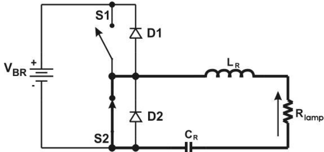
Fig.15.d. Fourth stage.
