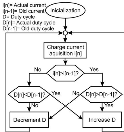
Fig. 9. MPPT algorithm implemented in the microcontroller.
