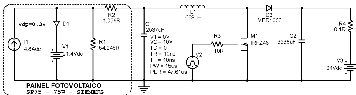
Fig. 11. The charge controller with the Siemens™ SP75 photovoltaic panel.
