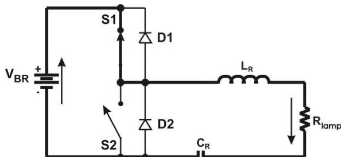
Fig.15.b. Second stage.
