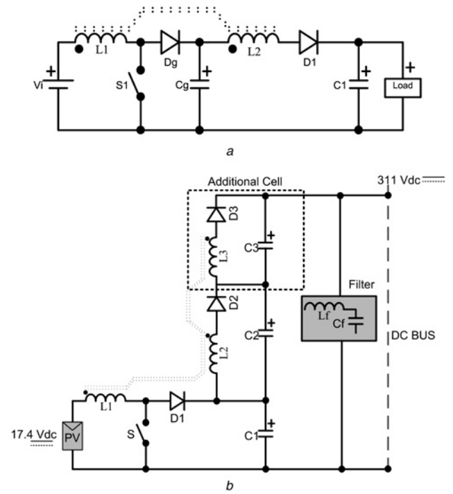
Fig. 1 High-voltage gain dc–dc converters based using coupled inductors a Topology studied in [33] b Proposed topology
